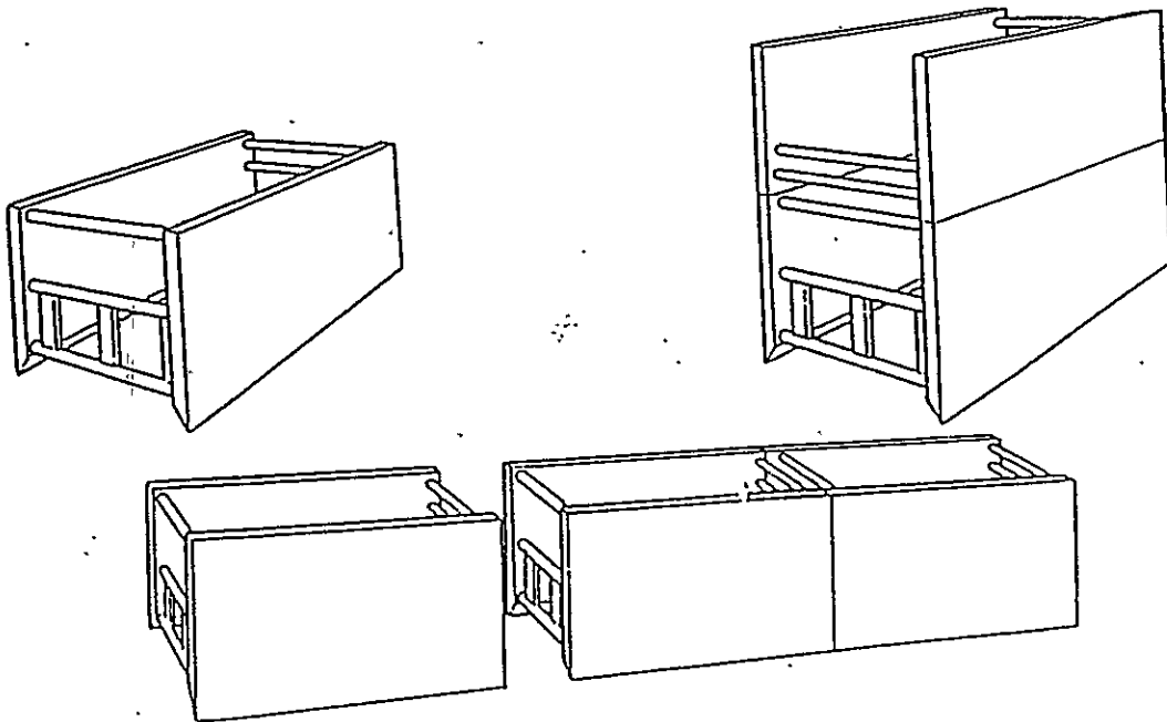
Figure 4. Trench Shields
